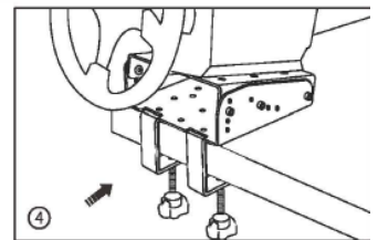
整体支架放置桌面,逆时针拧紧螺 Place the whole stand on the table and tighten the screw counterclockwise
